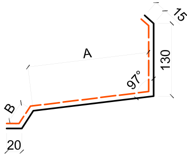
Sıva Dibi Profili / Roof to Wall Junction Profile
