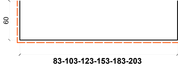
Soğuk Oda Zemin U Profili / Ground U Profile Cold Storag
